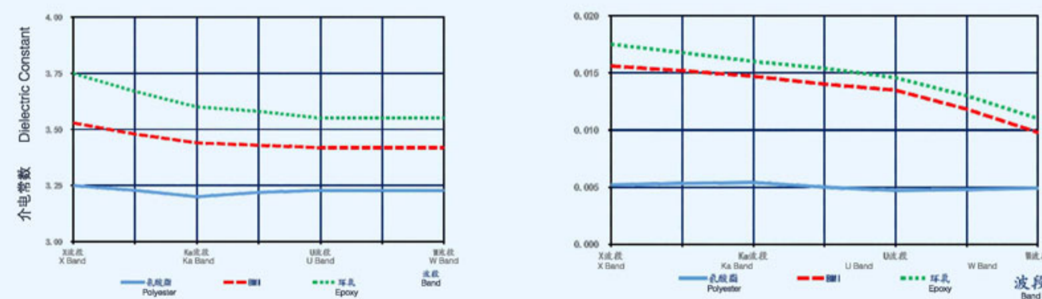
石英纤维在不同树脂体系下的宽频介电性能 Broadband dielectric properties of quartz fiber in different resin systems.
